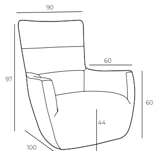
Chair with swivel mechanism MICA WITH SWIVEL
